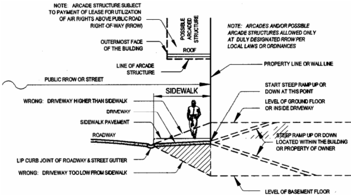
LONGITUDINAL SECTION OF DRIVEWAY
